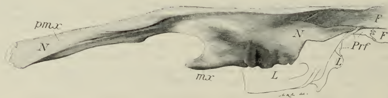
Figure 11. Right nasal of Edmontosaurus , Cat. No. 2289; internal aspect, obliquely from below; \frac{1}{2} natural size. F , frontal; L , lachrymal; mx , surface for maxillary; N , nasal; pmx , surface for upper limb of premaxillary; Prf , prefrontal.
